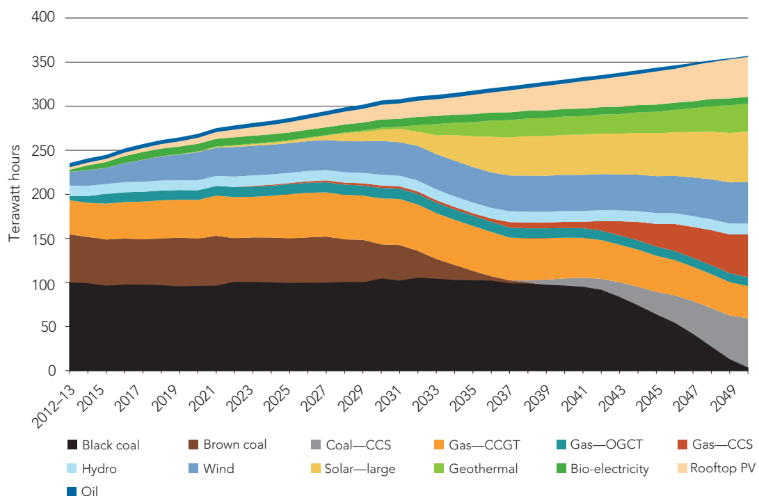
Figure 3.8: Australia's electricity generation mix to 2050—AEMO medium demand scenario
