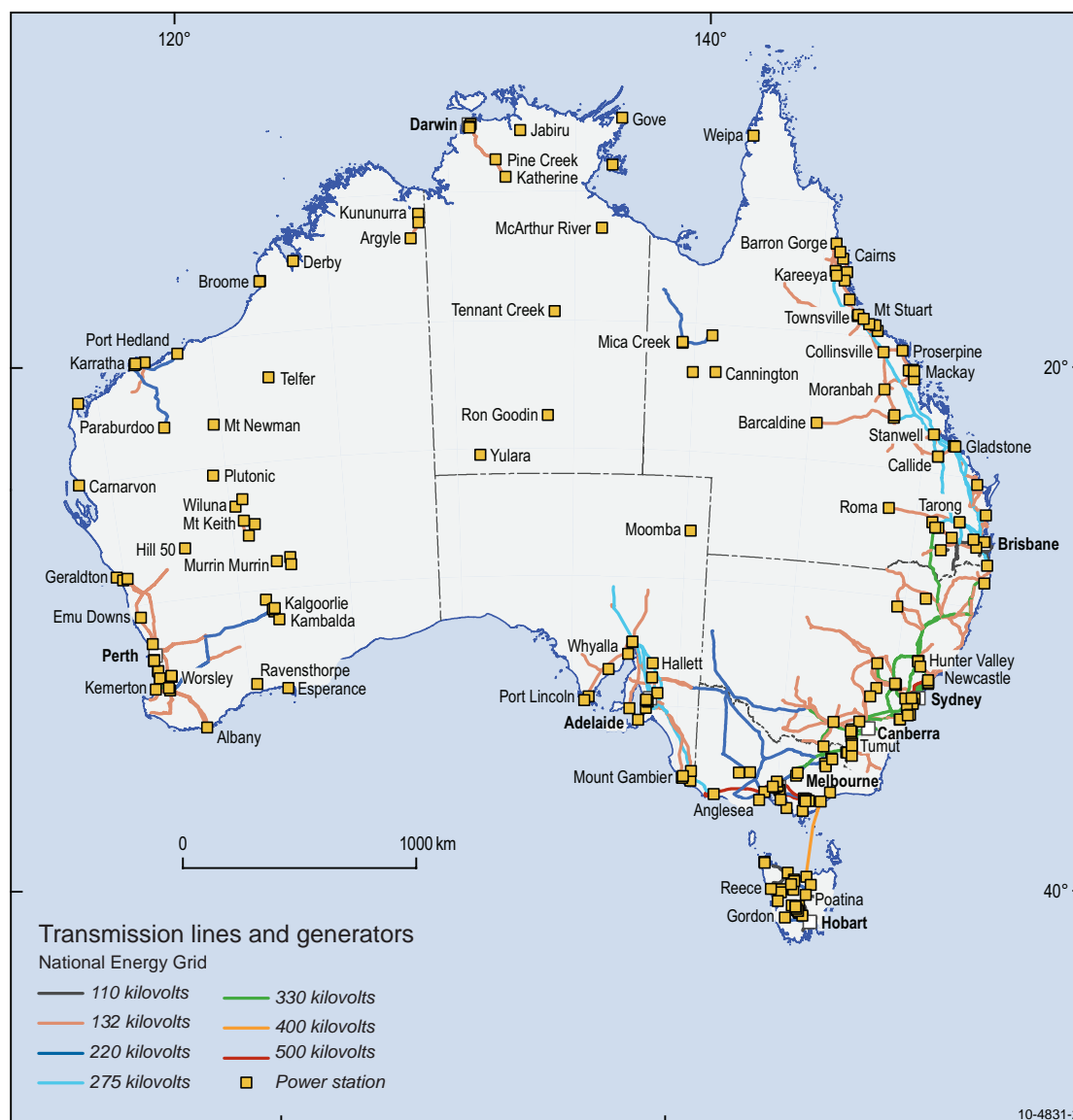
Figure 10.1: Australia's electricity systems
